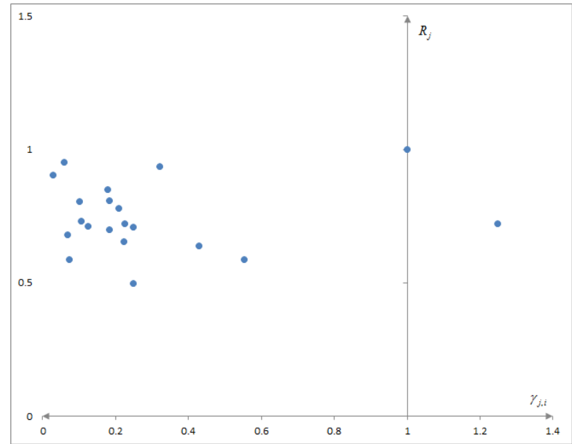
Figure 7: Local scale economies for DMU 12
