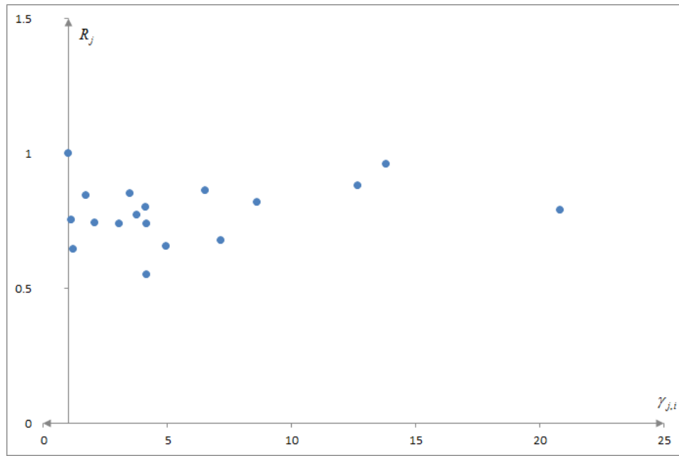
Figure 4: Local scale economies for DMU 5
