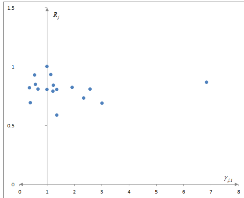
Figure 6: Local scale economies for DMU 8
