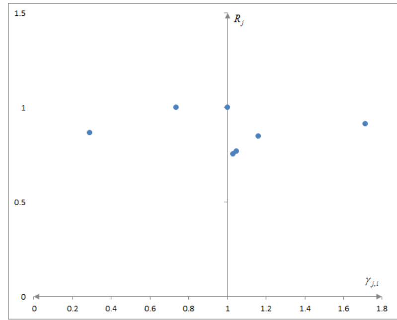
Figure. 5: Local scale economies for DMU 21
