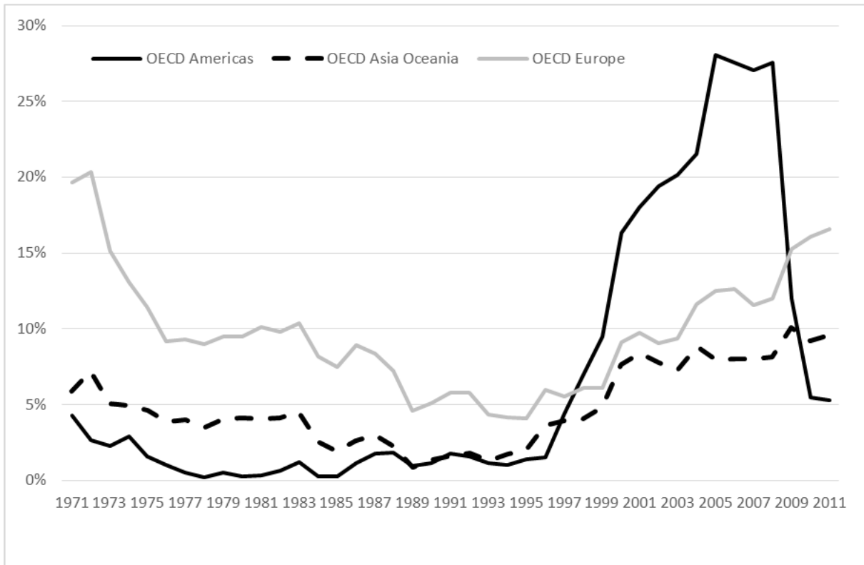
Figure 5: Overall inefficiency scores for groups
