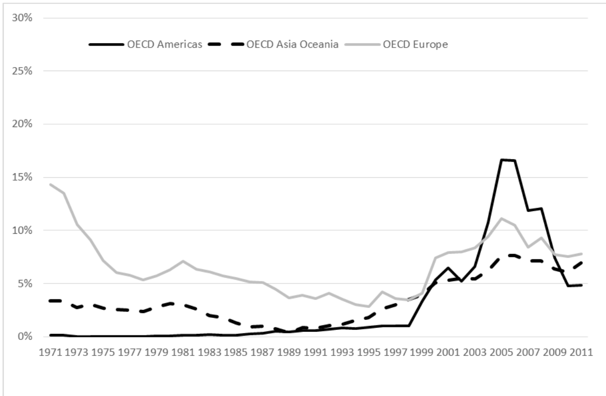
Figure 3: Technical inefficiency scores for groups
